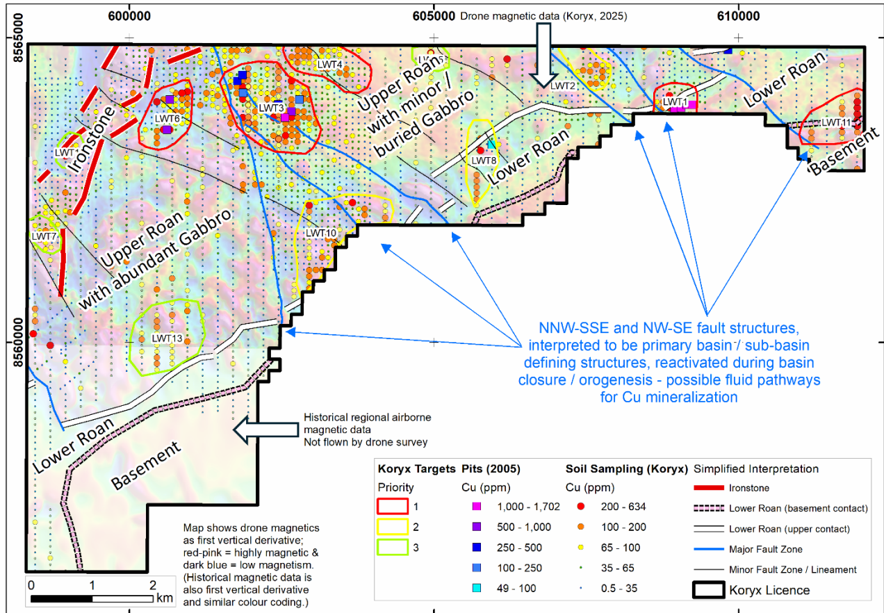
Figure 2: Summary map of results from 2025 work programs at Luanshya West; summary of targets identified and prioritised for drilling in 2026.
