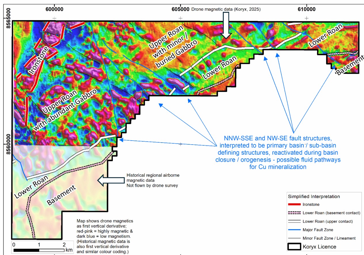
Figure 1: Results from 2025 drone-based magnetic data and simplified interpretation at Luanshya West.
